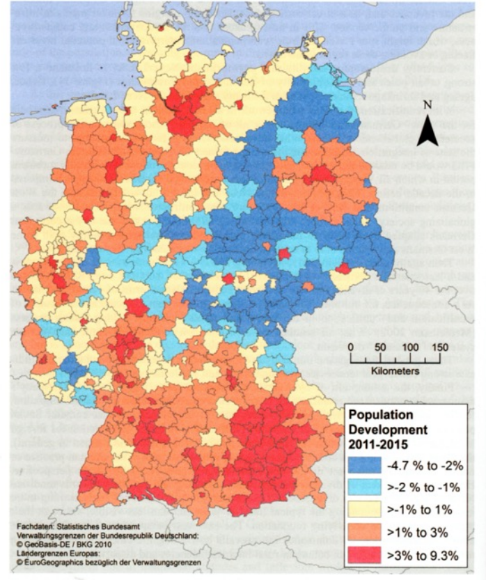
Figure 34: Recent total population development in Germany on the county level 2011-2015
