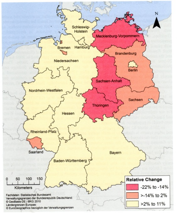
Figure 4: Relative change of population in German Länder 1991-2015
